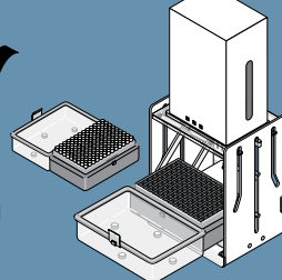
Remove filled rack and insert next empty rack into loader.
